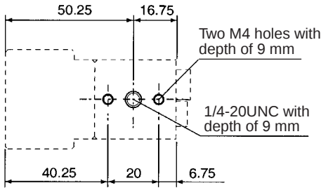
Mounting dimensions
