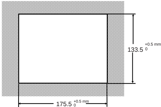
Panel opening dimensions
