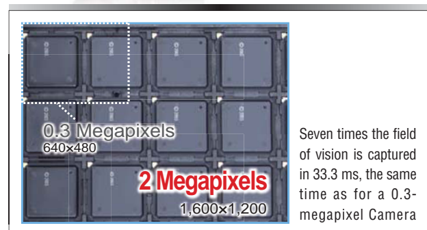
Camera 2 Megapixels
