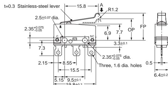
SS-3GL13P SS-01GL13P
