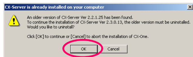
Uninstalling CX-Server
