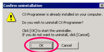
Uninstalling CX-Programmer
