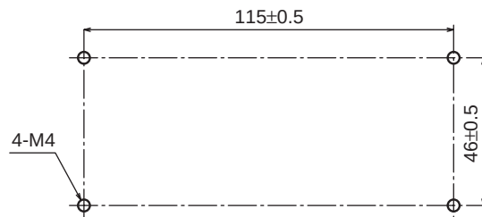
Mounting dimensions
