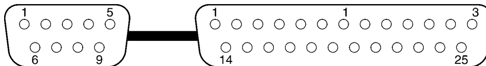
Connector Pin Arrangement when Viewed from the Controller
