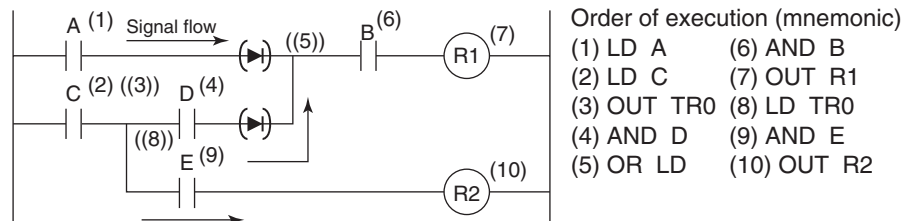
Circuit "a"
