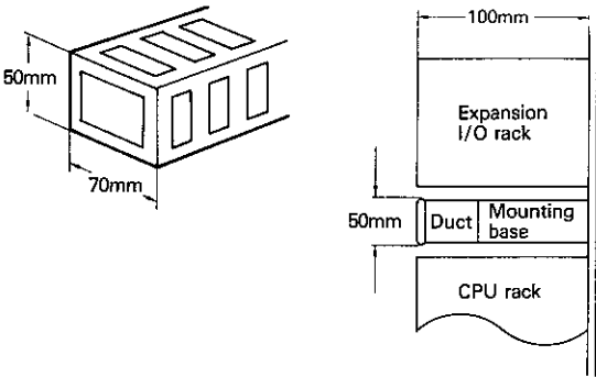
Standard duct dimensions
