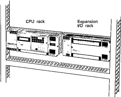
Horizontal mounting
