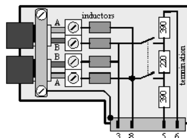
PROFIBUS-DP Connector with built-in inductors and termination
