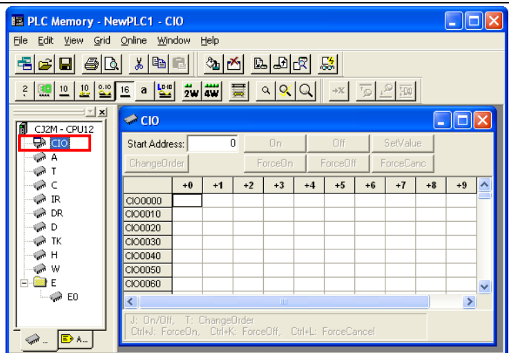
(PLC Memory Window)
