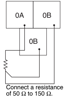
CRT1-TS04P Platinum-resistance thermometer input
