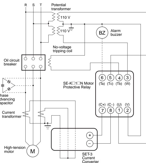
High-tension Motor No-voltage Tripping Circuit
