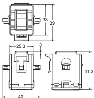
CT Through-hole Dimensions
