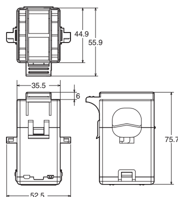
CT Through-hole Dimensions
