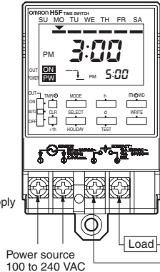
Surface Mounting Models H5F-FB
