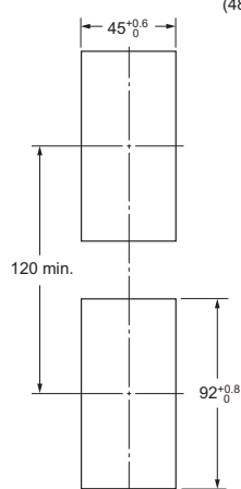
Mounted Separately
