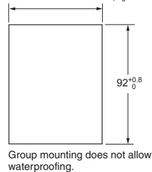
Group Mounted
