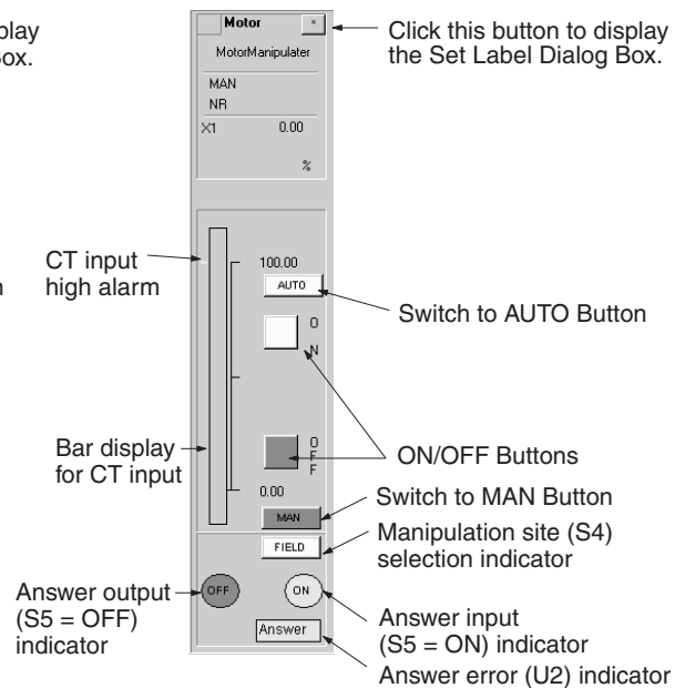
Motor Manipulation (222)
