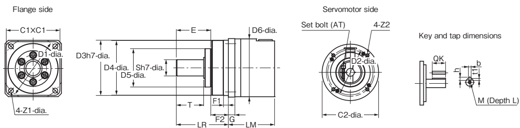
Outline Drawing 2
