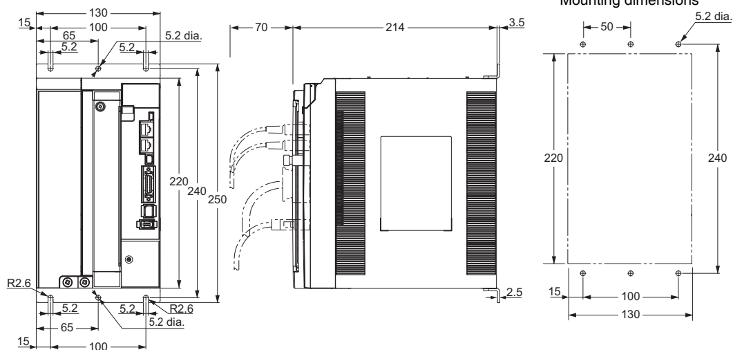
Mounting dimensions
