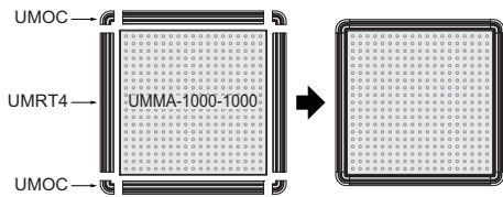
Example 1: Using a Single Safety Mat
