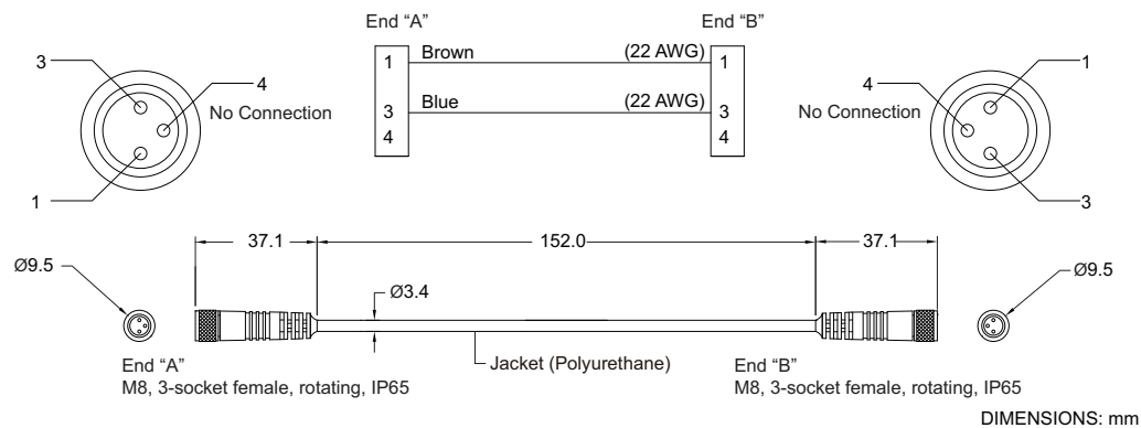
Fig. 6-6 UMA-CBL-3PFF-M8-0.15M
