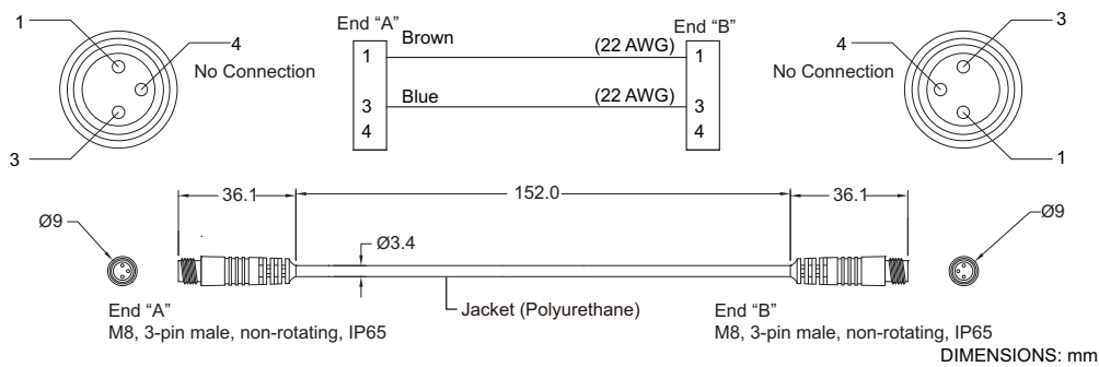
Fig. 6-5 UMA-CBL-3PMM-M8-0.15M
