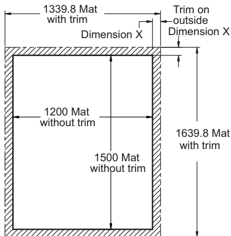
Fig. 4-6 Example Calculation
