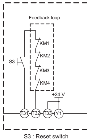
Wiring for manual reset mode
