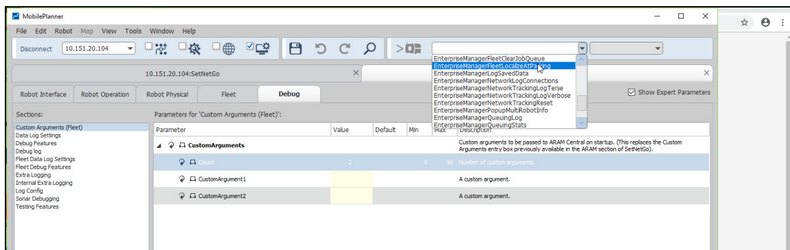
Figure 4-3. Command Drop-down.
