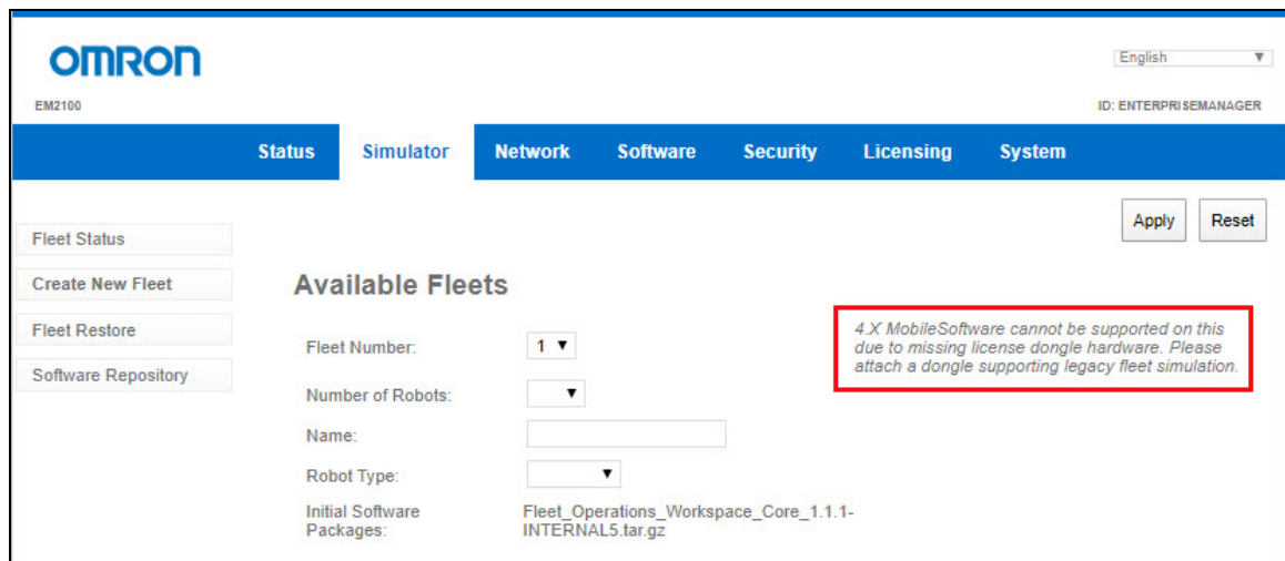
Figure 4-6. Available Fleet, Showing Legacy Software Note.
