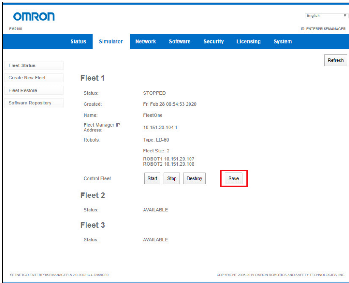
Figure 4-5. Save Button.
