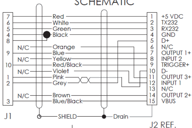
SCHEMATIC
