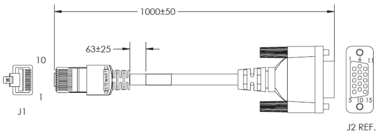
SCHEMATIC
