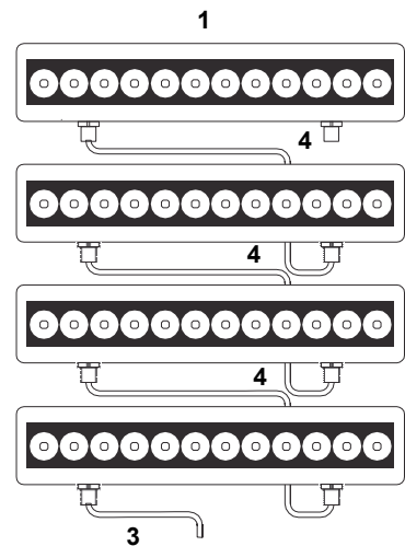
Figure D MAX Series Illuminator in a daisy chain configuration. See figures A, B, or C for the correct power supply and signal connections for your application.
