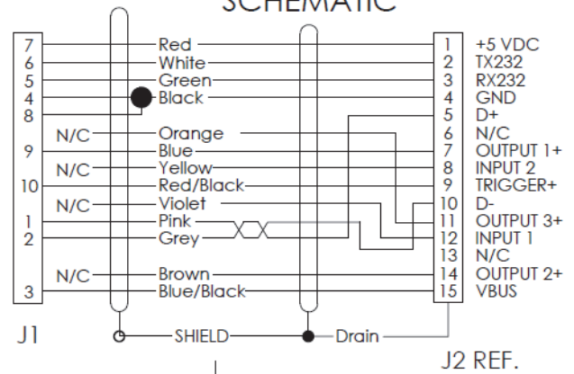
SCHEMATIC
