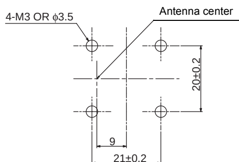
Mounting dimensions
