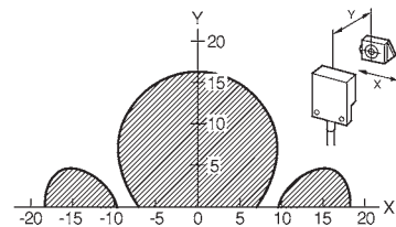
V600-HS61 + V600-D23P61
