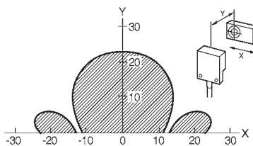
V600-HS61 + V600-D8KR12D
