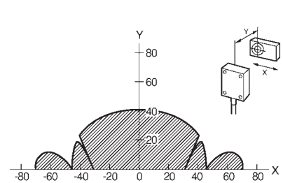
V600-HS67 + V600-D8KR13
