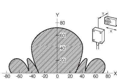
V600-HS67 + V600-D8KR12D
