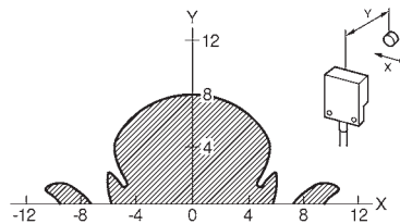
V600-HS61 + V600-D23P54
