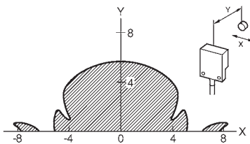
V600-HS61 + V600-D23P53
