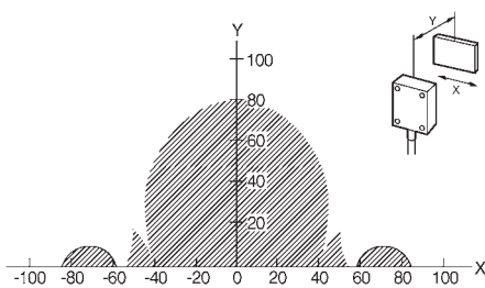
V600-HS67 + V600-D23P72
