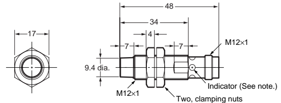
E2A-M12KN08-M1-□□/E2A-S12KN08-M1-□
