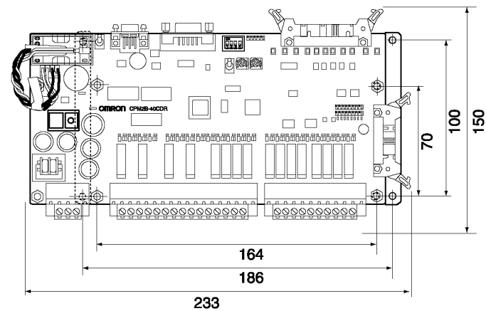
40-point CPU Board or Expansion I/O Board
