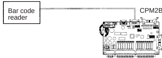
Inputting data from a bar code reader
