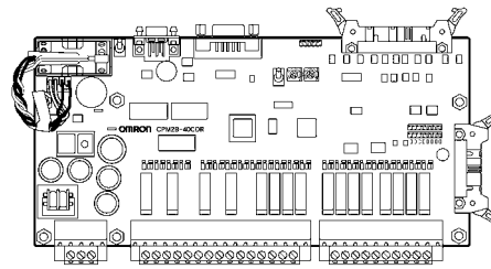
CPU Board with 40 I/O points (Relay outputs)
