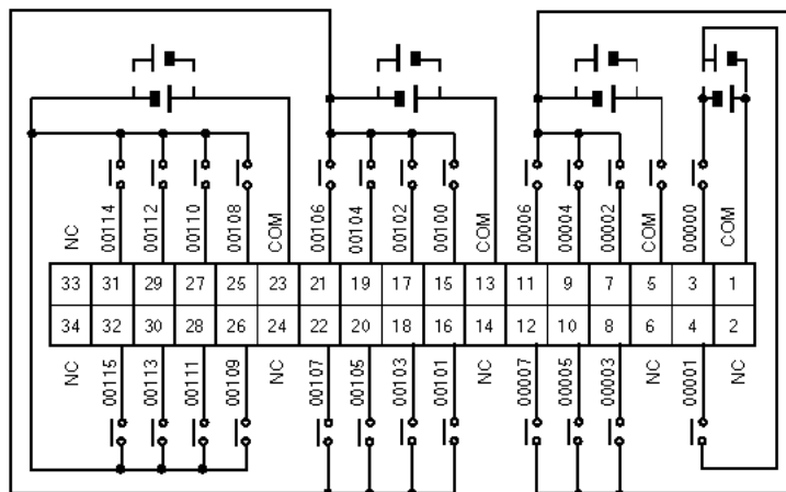
Input Connector
