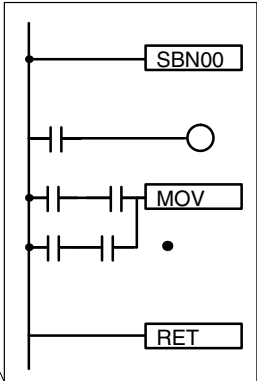
Interrupt program
