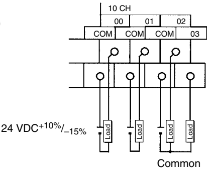
CPM1A-20CDT1-□(-V1)/CPM1A-20EDT1
