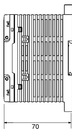
CPU Unit with AC Power
