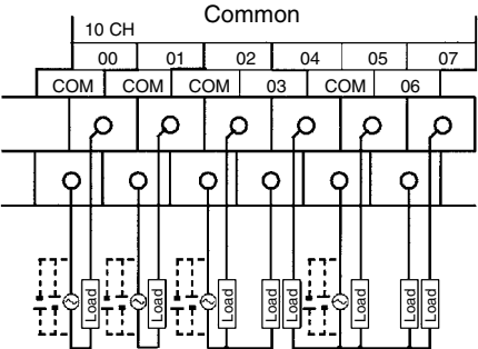
CPM1A-20CDR-□(-V1)/CPM1A-20EDR/20EDR1
