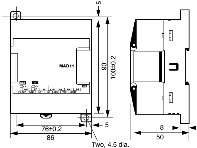
CPM1A-MAD11
