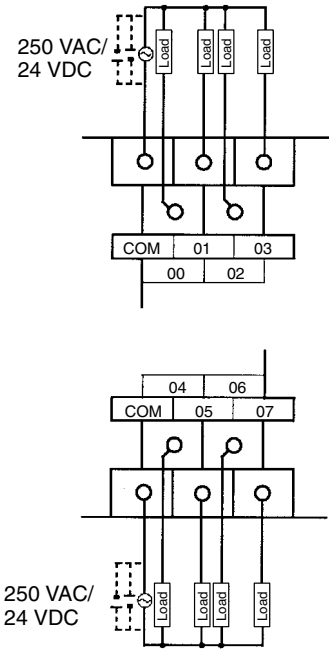
CPM1A-8ER
