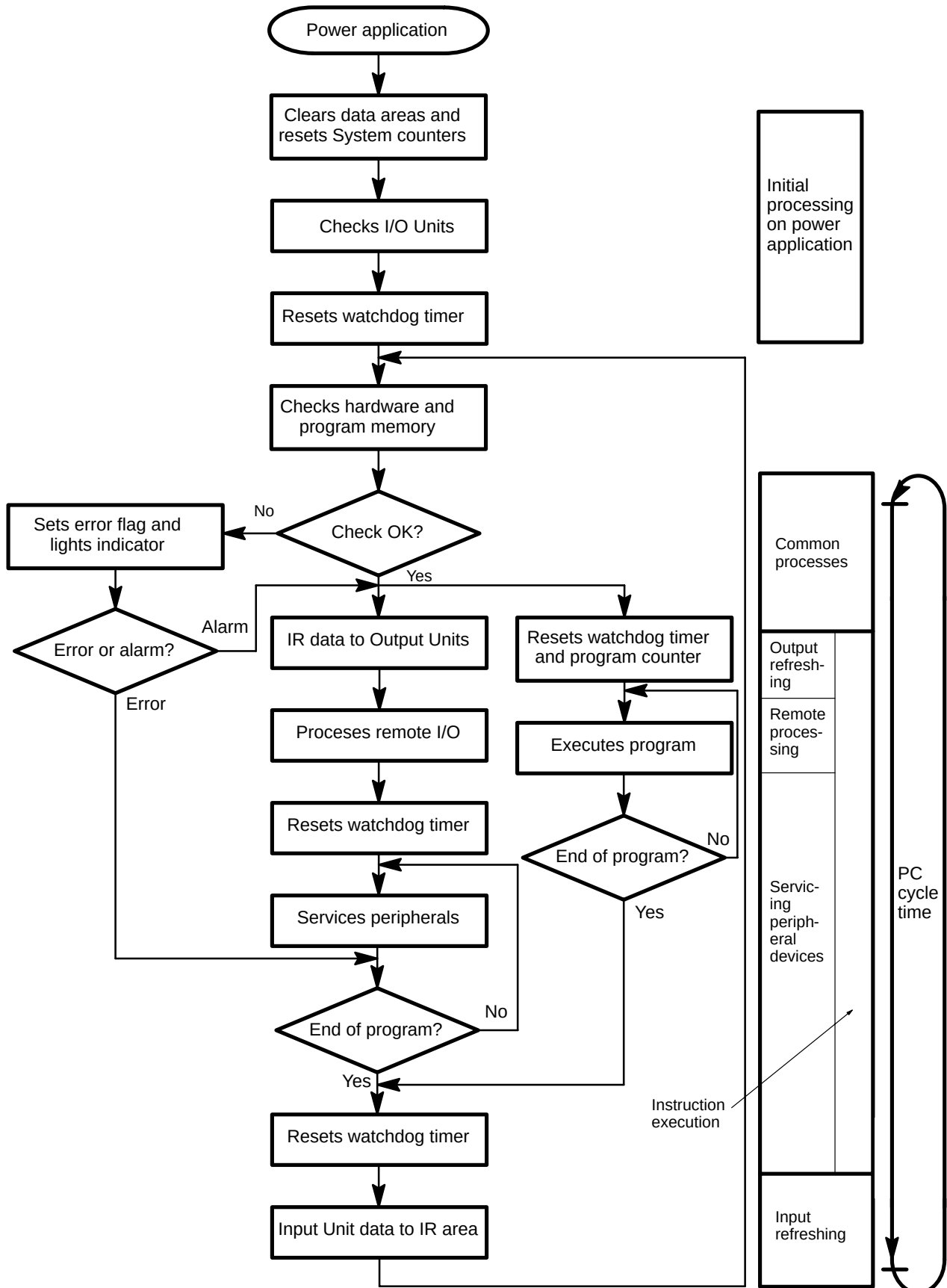
PC Operation Flowchart
