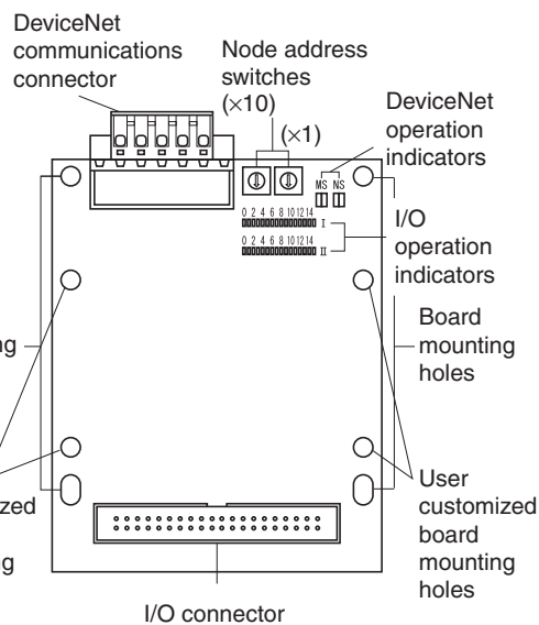
DRT2-ID32BV (NPN)/DRT2-ID32BV-1 (PNP)
