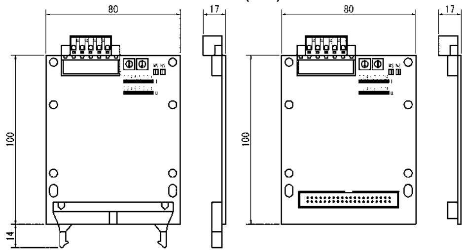
DRT2-MD32B (NPN)/DRT2-MD32B-1 (PNP) DRT2-MD32BV (NPN)/DRT2-MD32BV-1 (PNP)
