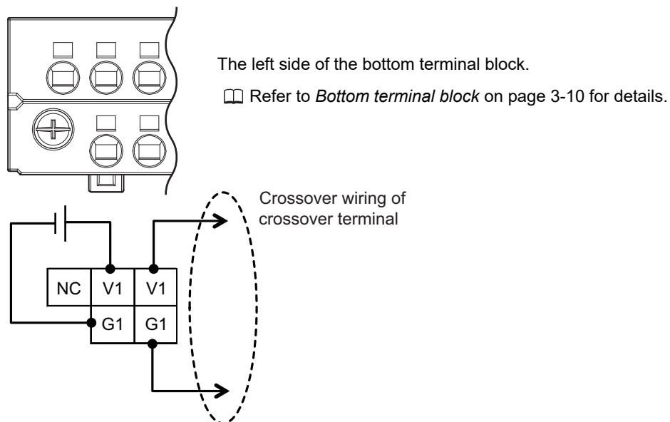
Output power supply terminal (Bottom terminal block)
