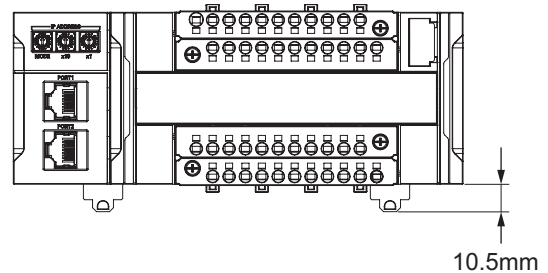
Unlocked position of DIN Track mounting hook
