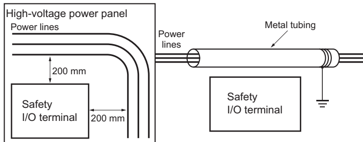
Example: Separating safety I/O terminal from Power Lines
