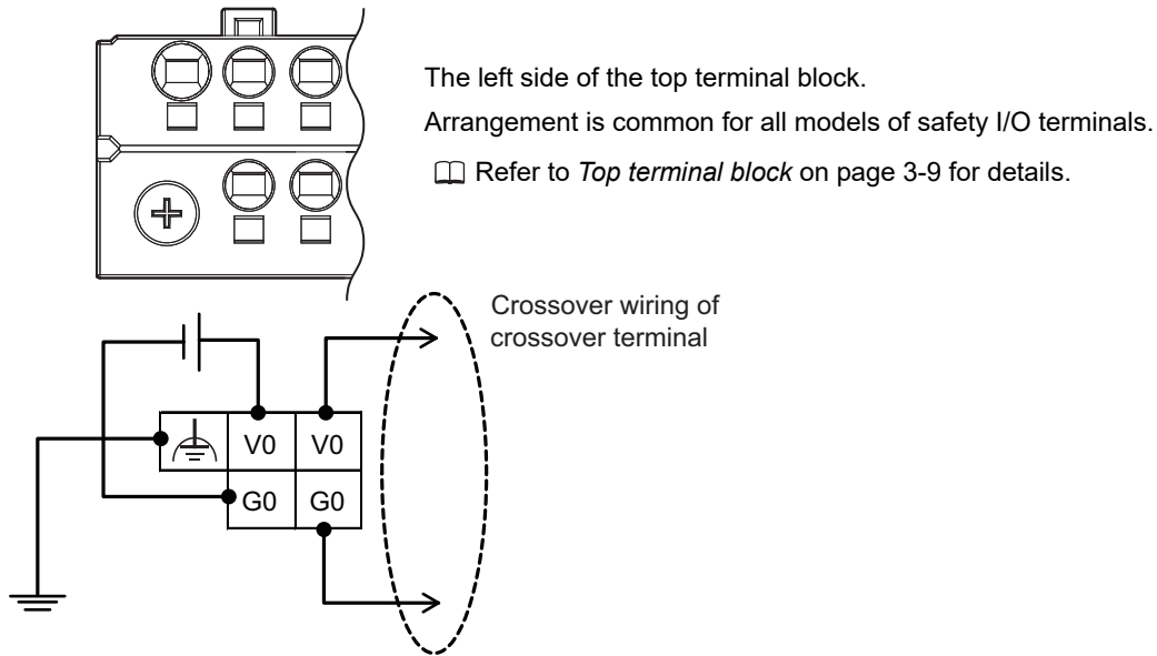
Unit power supply terminal (Top terminal block)
