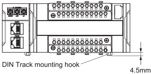
Locked position of DIN Track mounting hook
