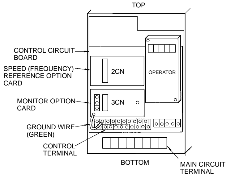
Option Card Installing Position
