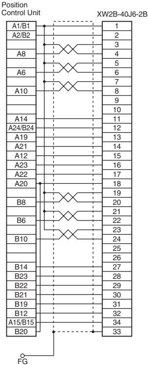
XW2Z-100J-A9 (for the R7D-AP and R88D-UEP0000)
