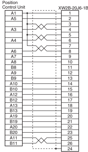
XW2Z-100J-A4 (for the R7D-AP and R88D-UEP0000)
