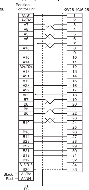
XW2Z-050J-A13 (for the R7D-AP and R88D-UEP0000)
