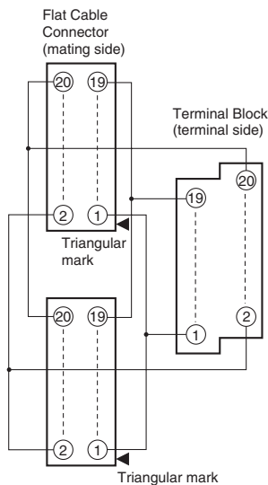
Wiring Diagram
